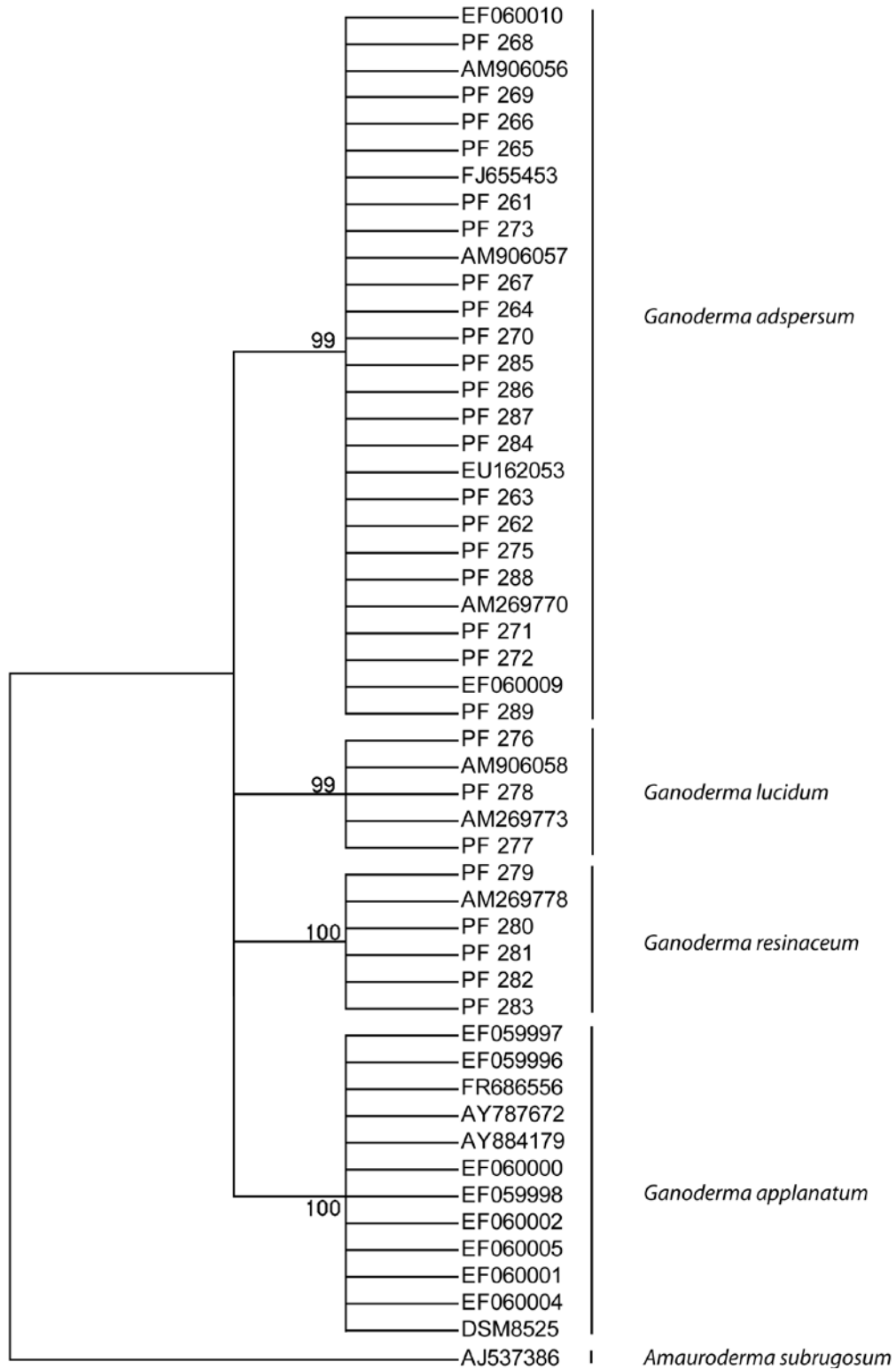
Figure 2. Phylogenetic tree, obtained by maximum parsimony analysis (MP), based on comparison of ITS region sequences of Ganoderma spp. (Tables 1 and 2). Values at nodes are confidence levels (1000 bootstraps).
